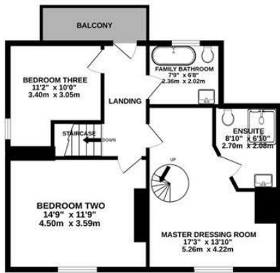
1ST FLOOR 624 sq.ft. (58.0 sq.m.) approx.
